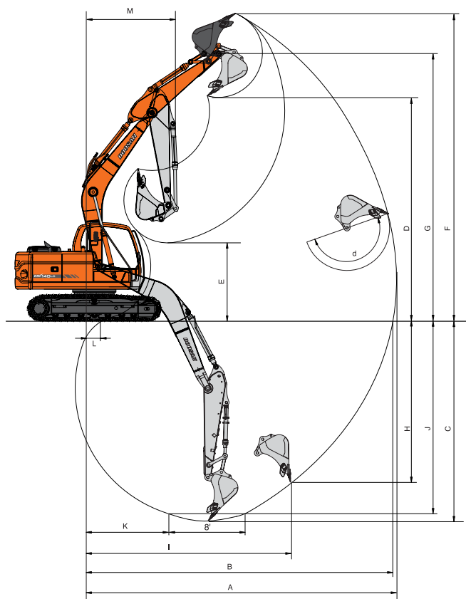
[ One-piece Boom ]
