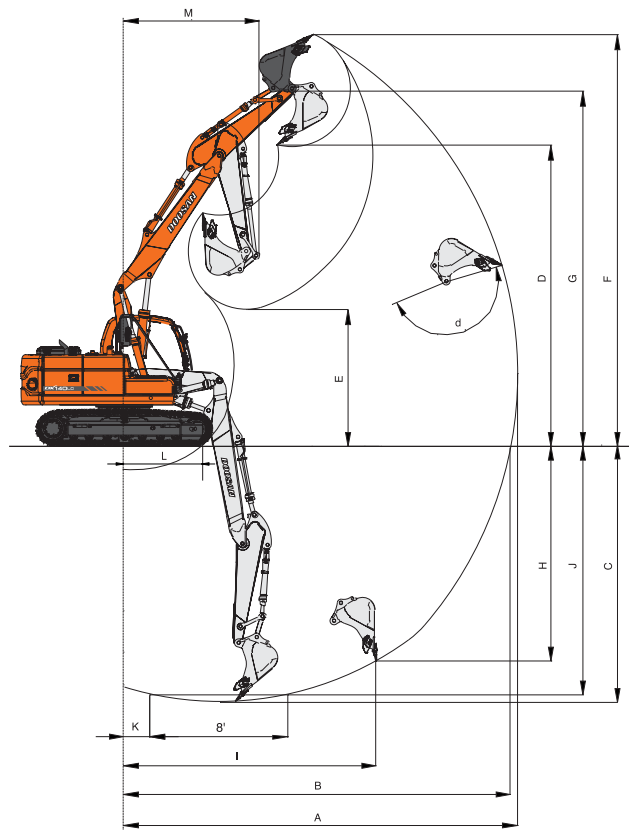
[ Two-piece Boom ]
